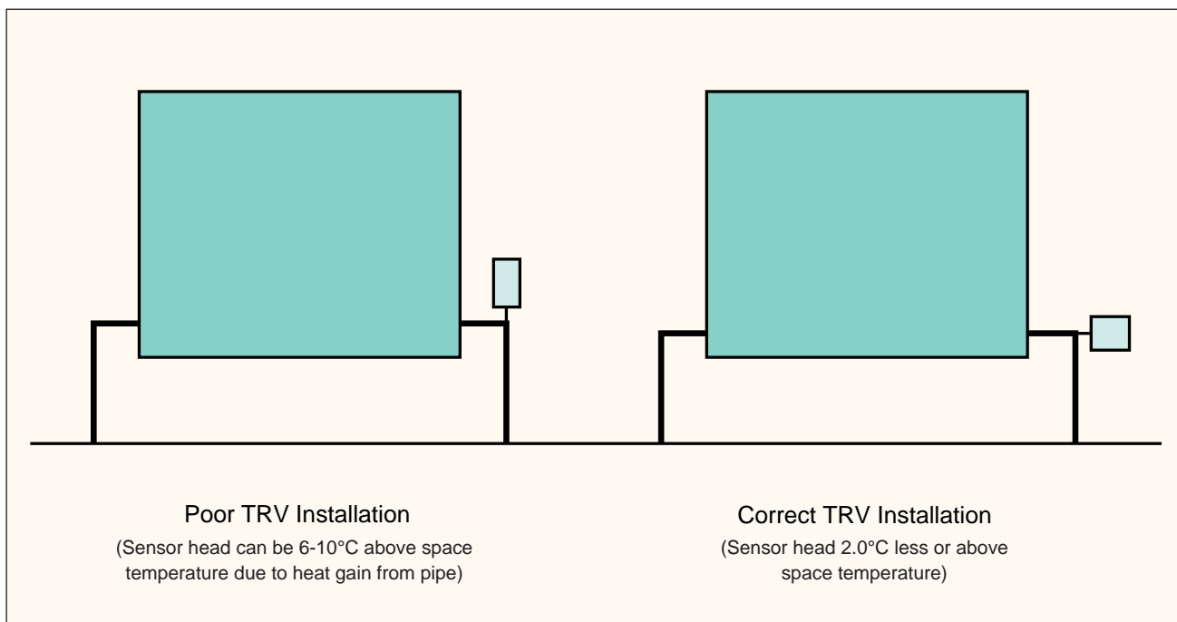
Figure 10 TRV installation
