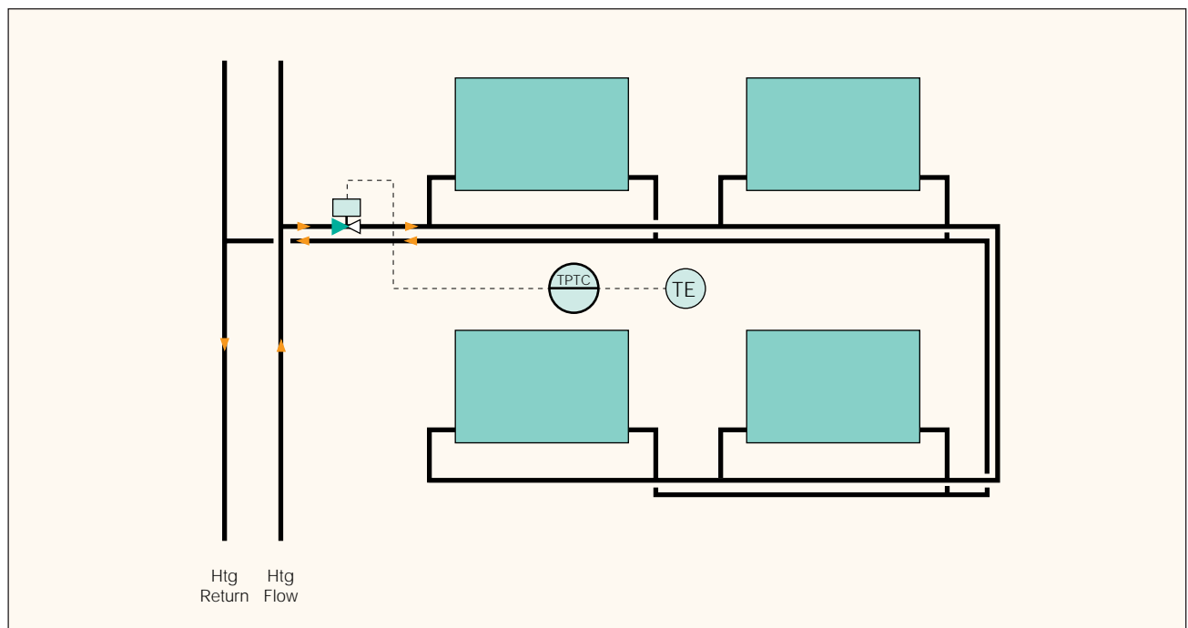
Figure 12 Time proportioning control
