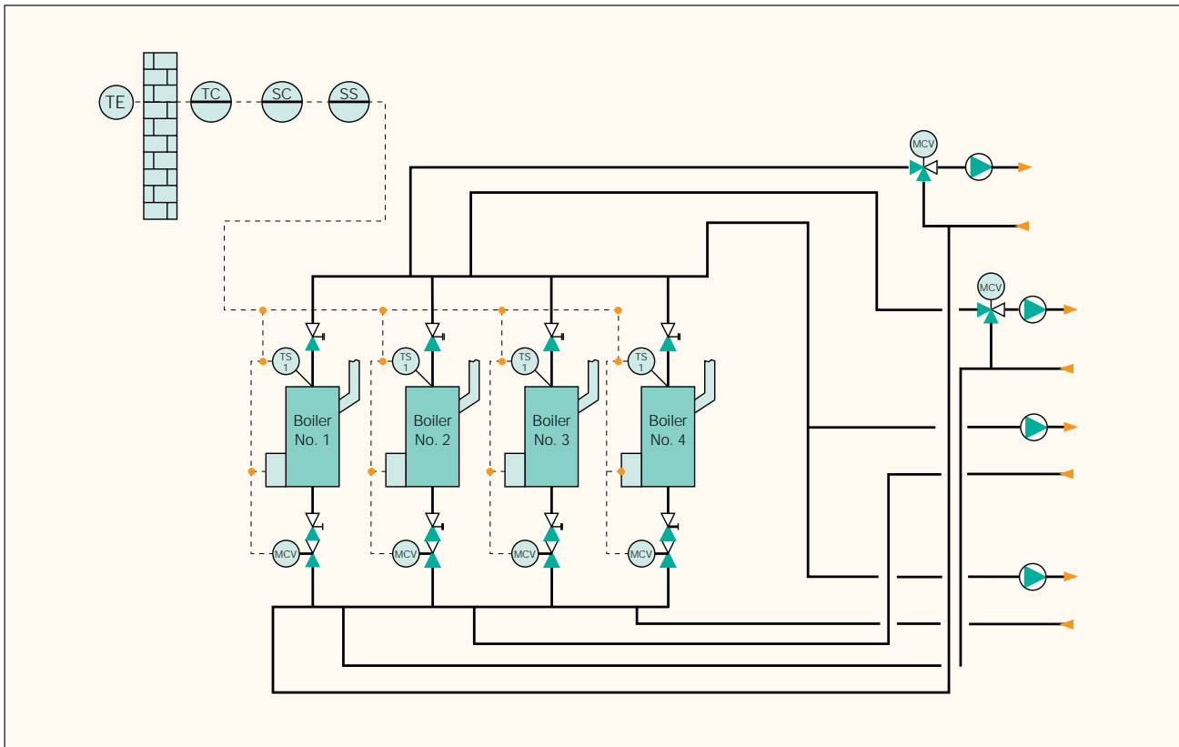
Figure 6 Problematic system
