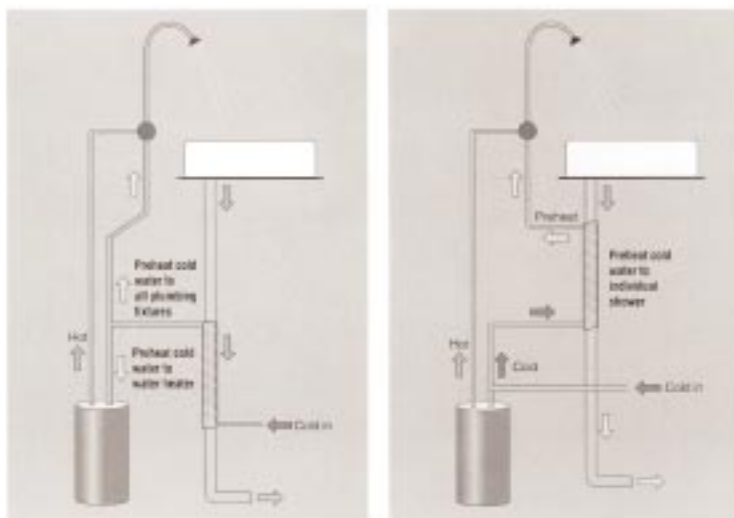
FIGURE 7 GFX HEAT RECOVERY SYSTEM
