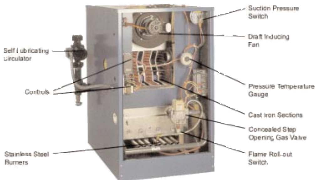
GAS-FIRED BOILER
