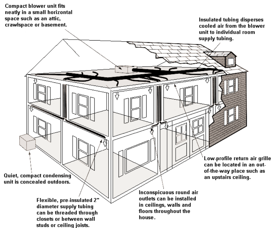
MINI-DUCT DISTRIBUTION SYSTEM
