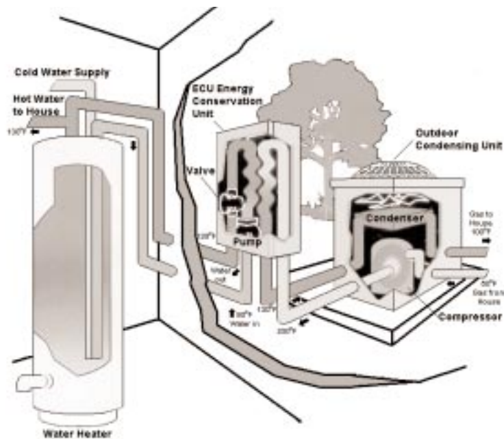
FIGURE 6 HOT WATER DESUPERHEATER
