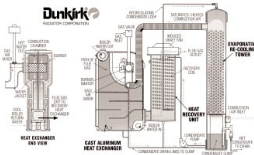
FIGURE 5 QUANTUM LEAP CONDENSING BOILER
