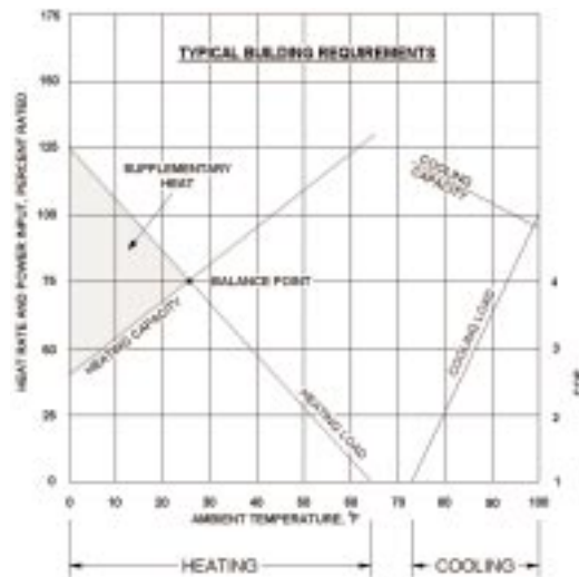
FIGURE 2 HEAT PUMP CAPACITY AND AMBIENT TEMPERATURE RELATIONSHIP
