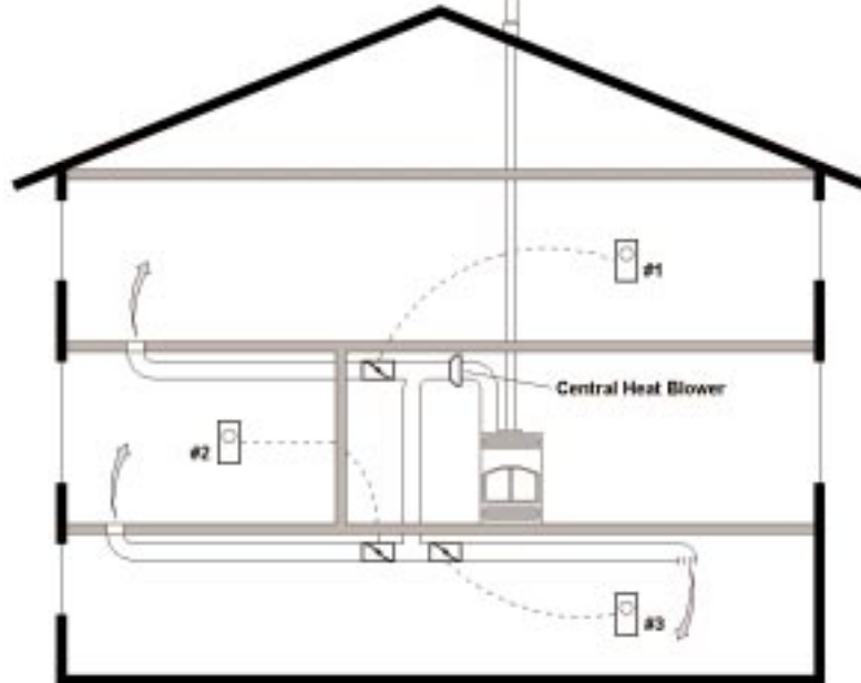
FIGURE 8 DUCTED FIREPLACE
