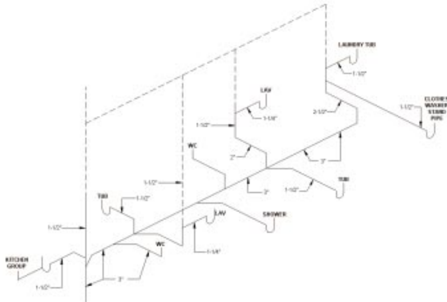
FIGURE 6 CIRCUIT VENT WITH ADDITIONAL NON-CIRCUIT VENTED FIXTURES
