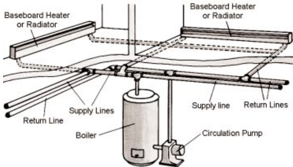
FIGURE 2 TYPICAL HYDRONIC DISTRIBUTION SYSTEM
